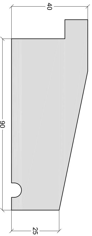
Projecting Cill 1:1 on A4
