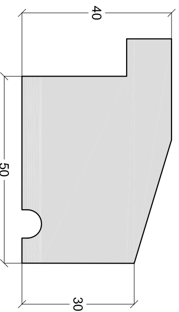
Projecting Cill 1:1 on A4
