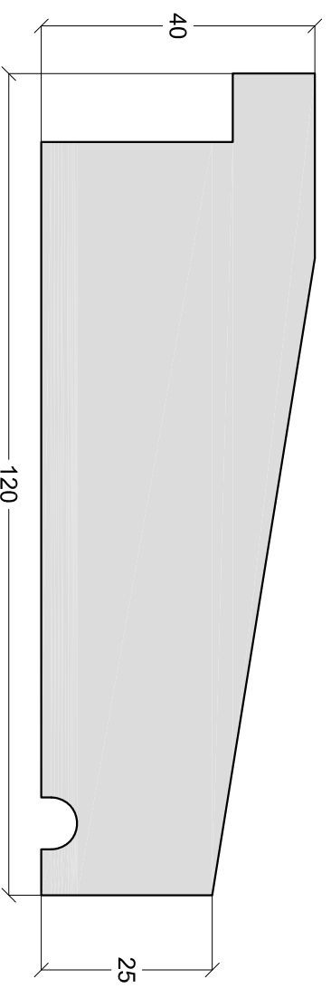
Projecting Cill 1:1 on A4
