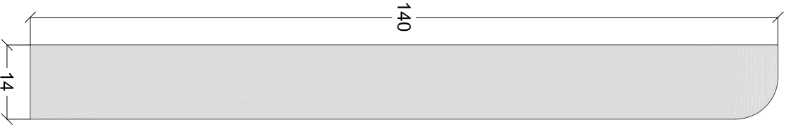
Skirting Board 99 B 1:1 on A4
