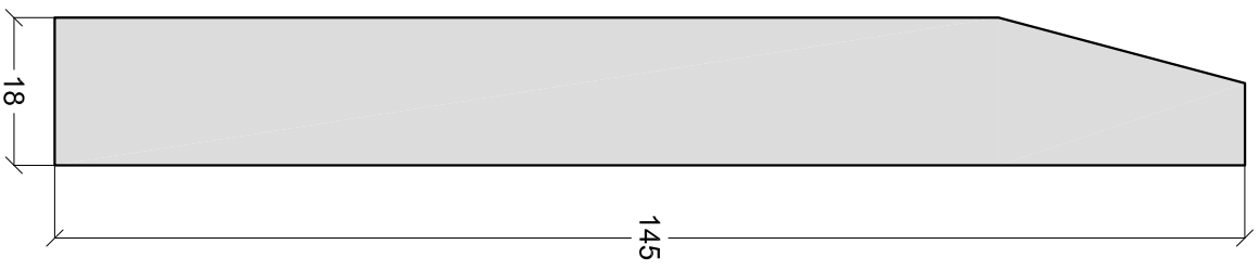
Skirting Board 95 B 1:1 on A4
