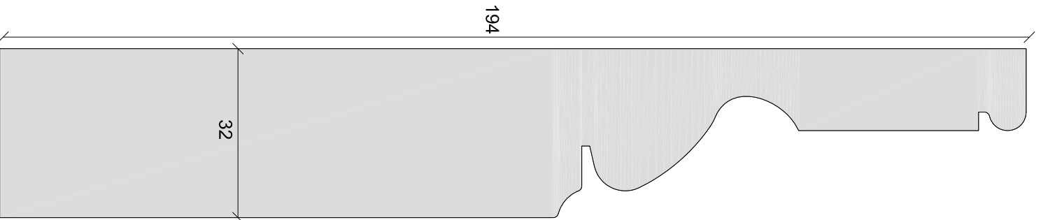
Skirting Board 16 1:1 on A4
