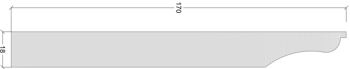
Skirting Board 15 B 1:1 on A4
