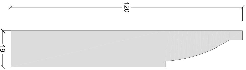
Skirting Board 11 C 1:1 on A4
