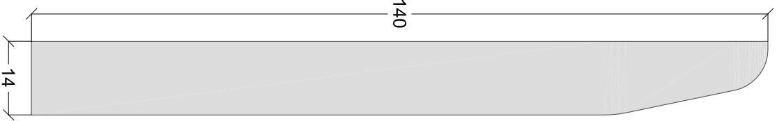
Skirting Board 09 B 1:1 on A4
