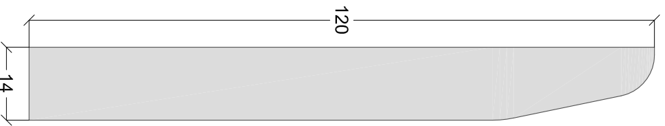
Skirting Board 09 A 1:1 on A4
