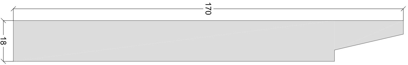
Skirting Board 08 D 1:1 on A4
