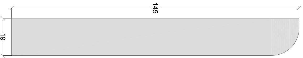
Skirting Board 06 C 1:1 on A4
