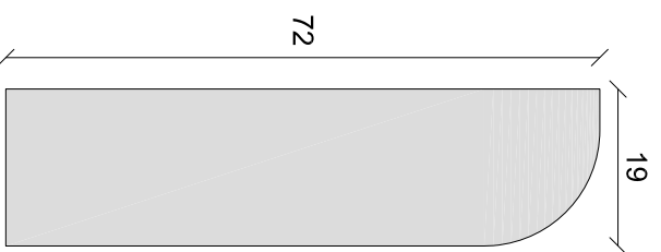
Skirting Board 06 1:1 on A4
