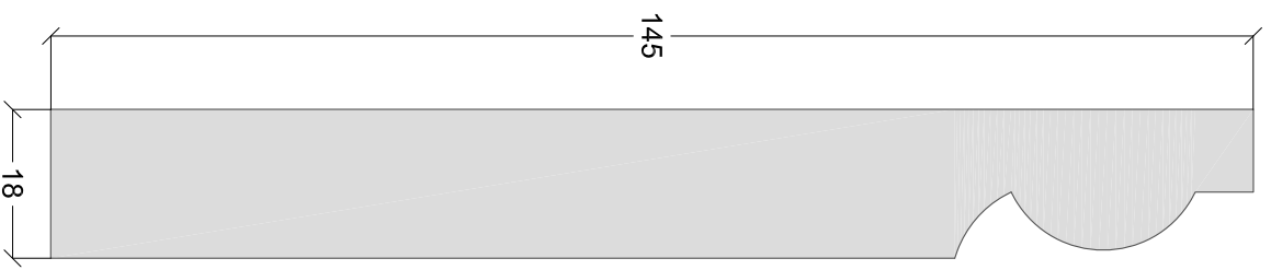
Skirting Board 02 A 1:1 on A4
