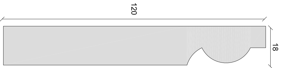
Skirting Board 02 1:1 on A4
