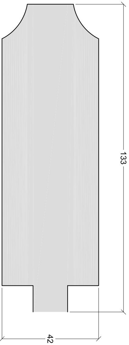
Roof Rafter 02 1:1 on A4
