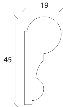
Picture Rail 1:1 on A4
