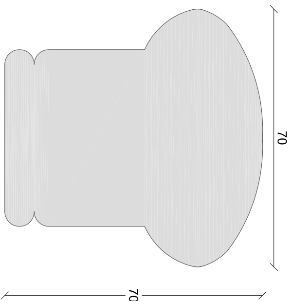
Handrail 09 1:1 on A4
