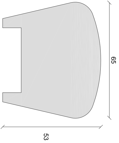
Handrail 08 1:1 on A4
