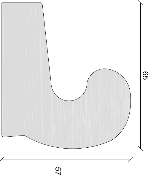
Handrail 07 1:1 on A4
