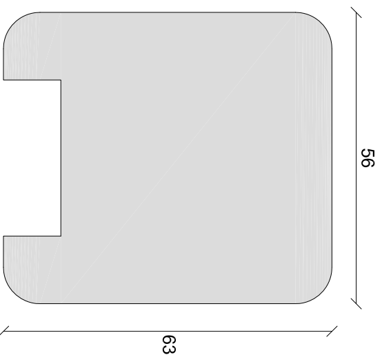
Handrail 01 1:1 on A4
