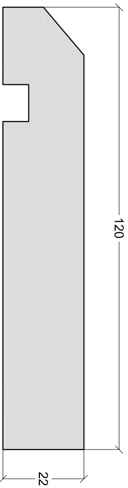
Fascia Board 02 1:1 on A4
