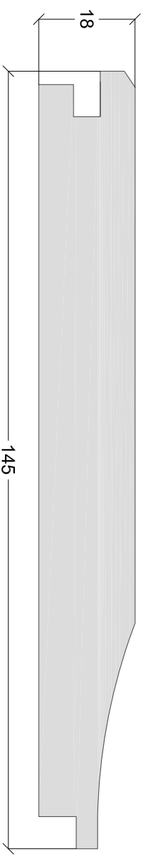
Cladding 01 B 1:1 on A4
