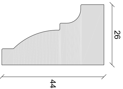
Cover Fillet 02 1:1 on A4
