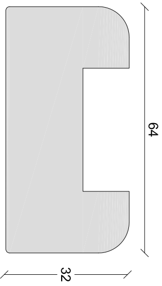
Baserrail 08-1 1:1 on A4
