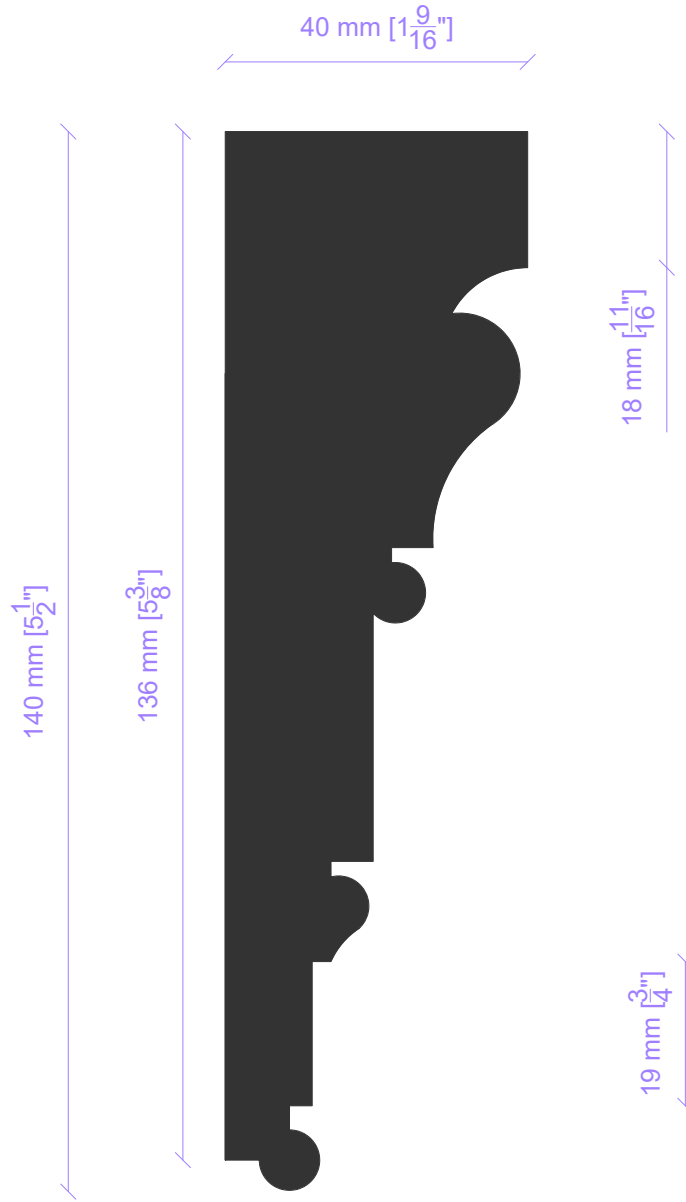
Architrave 19 1:1 on A4
