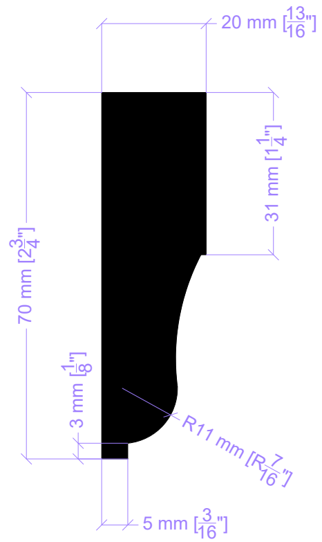
Architrave 15 A 1:1 on A4
