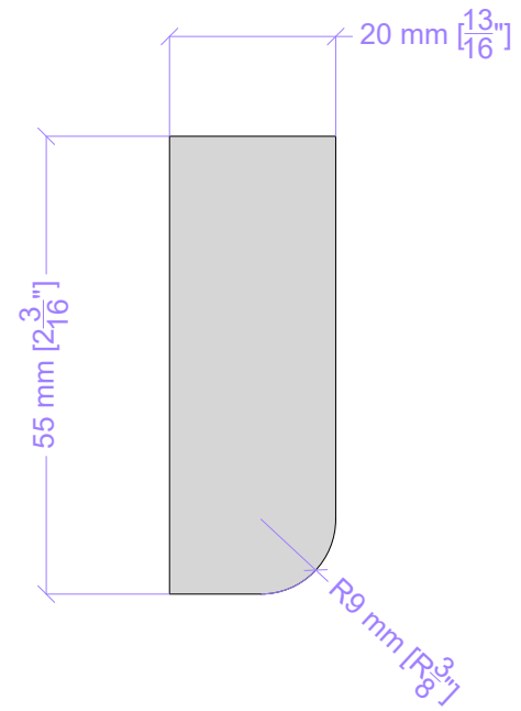
Architrave 14 A 1:1 on A4
