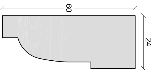
Architrave 11 1:1 on A4
