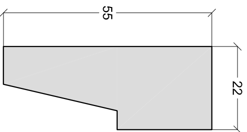
Architrave 08 B 1:1 on A4
