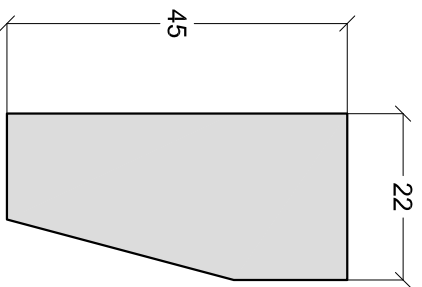
Architrave 05 B 1:1 on A4
