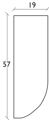
Architrave 1:1 on A4
