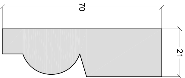
Architrave 03 A 1:1 on A4
