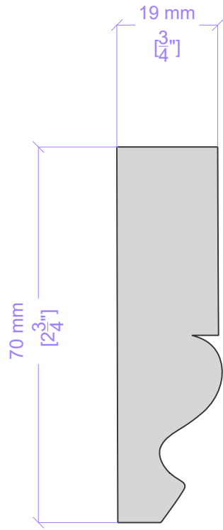
Architrave 01G2 1:1 on A4
