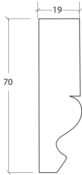
Architrave 1:1 on A4
