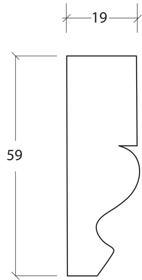
Architrave 01 A 1:1 on A4
