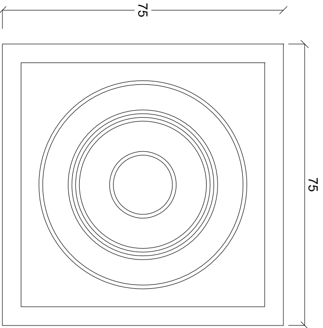
Architrave Block 04 1:1 on A4
