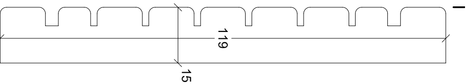
Architrave Block 01 1:1 on A4
